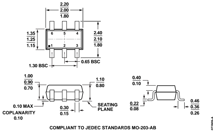
Figure 43. 6-Lead Thin Shrink Small Outline Transistor Package [SC70] (KS-6) Dimensions shown in millimeters
